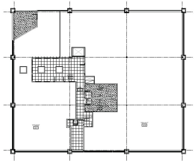
Second Floor
